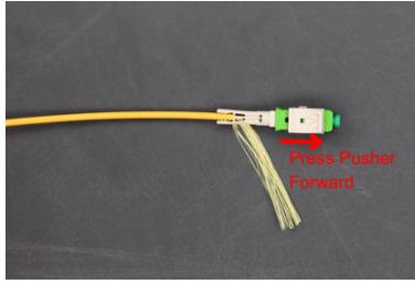
Step 13: Press the pusher forward to lock the fiber.
