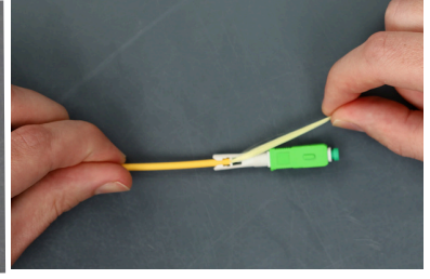
Step 15: On the opposite side, straighten the Kevlar.
