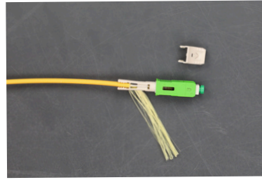
Step 14: Remove the pusher. **Note: Do NOT discard the pusher 1
