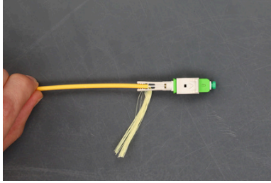
Step 12: Press the outer jacket into the slot.
